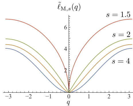
Fig. 5. The graphs of the functions \tilde{\ell}_{M,s} on the interval [-\pi, \pi] . The parameter s is varied from top to the bottom as 1.5, 2, 2.5 (not labelled) and 4.
