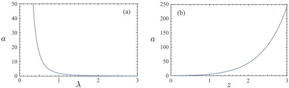
Fig. 4. The parameter dependence of a for (a) the Laplace-transformed and (b) the factorial-transformed k -path Laplacian.
