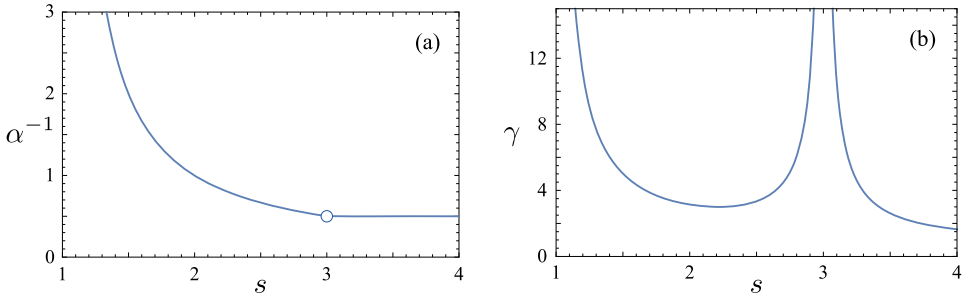
Fig. 7. The s -dependence of (a) 1/\alpha and (b) \gamma .
