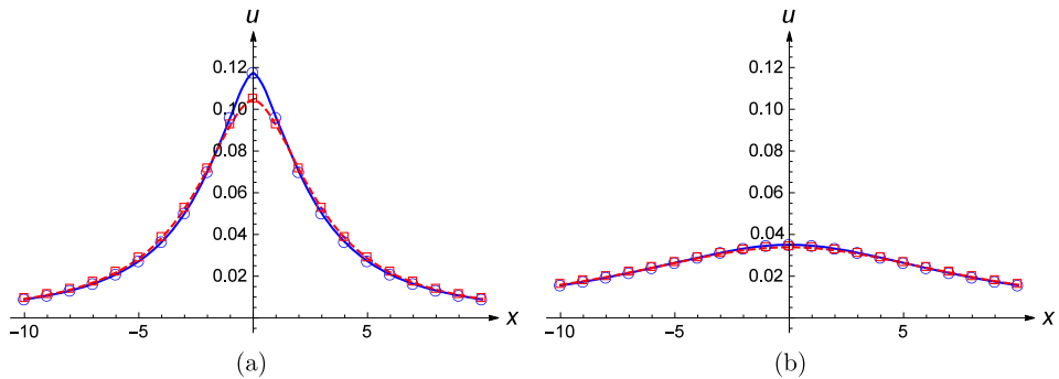
Fig. 8. The solutions of (6.1), (6.2) for L = \tilde{L}_{M,s} (blue solid line with circles) and for L = cL_1^a (red dashed line with squares) for t = 1 (a) and t = 3 (b). (For interpretation of the references to colour in this figure legend, the reader is referred to the web version of this article.)
