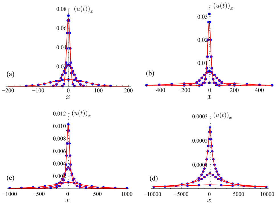
Fig. 6. The time evolution of the density profile under the Mellin-transformed k -path Laplacian: (a) s = 4 for t = 10, 100, 1000 from high to low; (b) s = 2.5 for t = 10, 100, 1000 from high to low; (c) s = 2 for t = 10, 30, 100 from high to low; (d) s = 1.5 for t = 10, 20, 40 from high to low. In every panel, the blue dots indicate the result of numerical integration of (6.5) with \ell = \tilde{\ell}_{M,s} , whereas the red curves indicate the asymptote (6.19). (For interpretation of the references to colour in this figure legend, the reader is referred to the web version of this article.)
