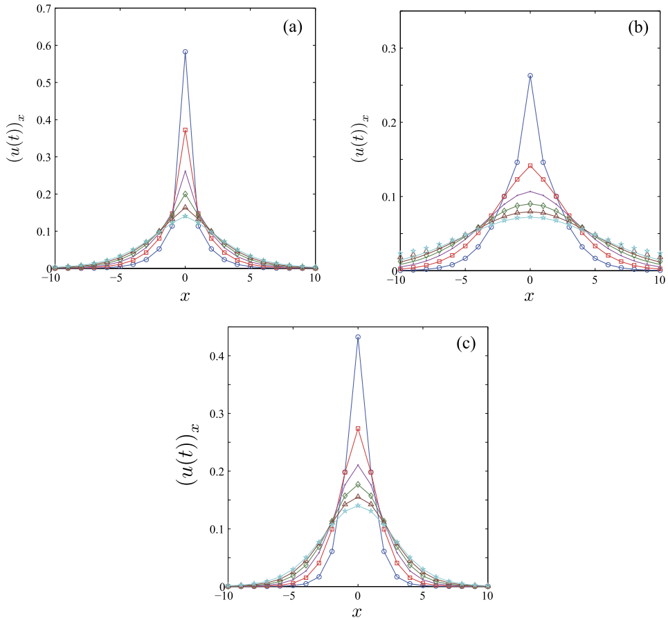
Fig. 2. The particle density (u(t))_x as a function of x for the transformed k -path Laplacians for a linear chain with 21 nodes. The symbols indicate the results obtained from the simulations of the linear chain and the solid lines represent the values obtained analytically from Theorem 5.2 for different time: t = 0.5 (circles), t = 1.0 (squares), t = 1.5 (dots), t = 2.0 (rhombus), t = 2.5 (triangles), t = 3.0 (stars). (a) Laplace transform with \lambda = 1 . (b) Factorial-transform with z = 1 . (c) Mellin-transform with s = 4 .
