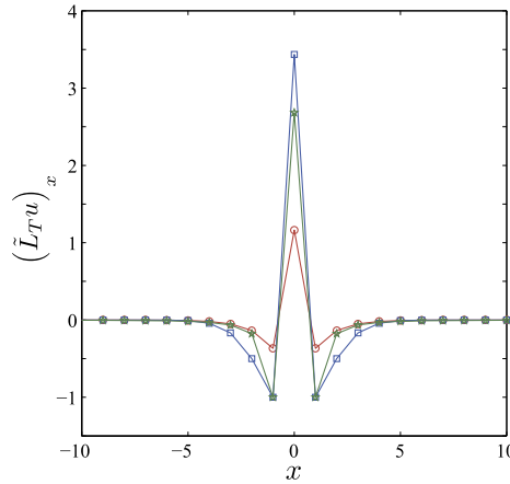
Fig. 1. Plot of the particle density at the different nodes of a linear path with 21 nodes obtained from the Laplace (circles), factorial (squares) and Mellin (stars) transformed k -path Laplacians with \lambda = 1 , z = 1 and s = 2.5 , respectively.
